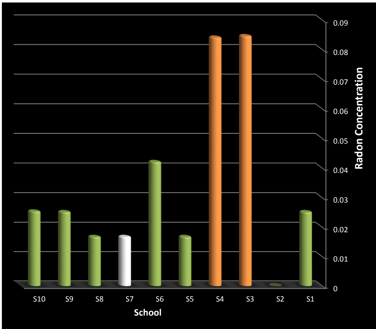
Fig. 2. Differences in radon gas concentrations in drinking water samples in the winter season.
